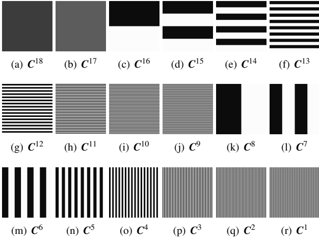
Figure 3: The 18 chosen cipher images for determining Y .
